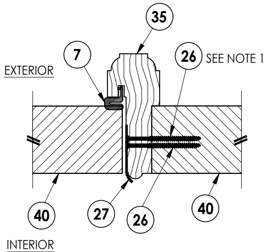
4 6 HORIZONTAL CROSS SECTION Inswing shown (Outswing similar)
