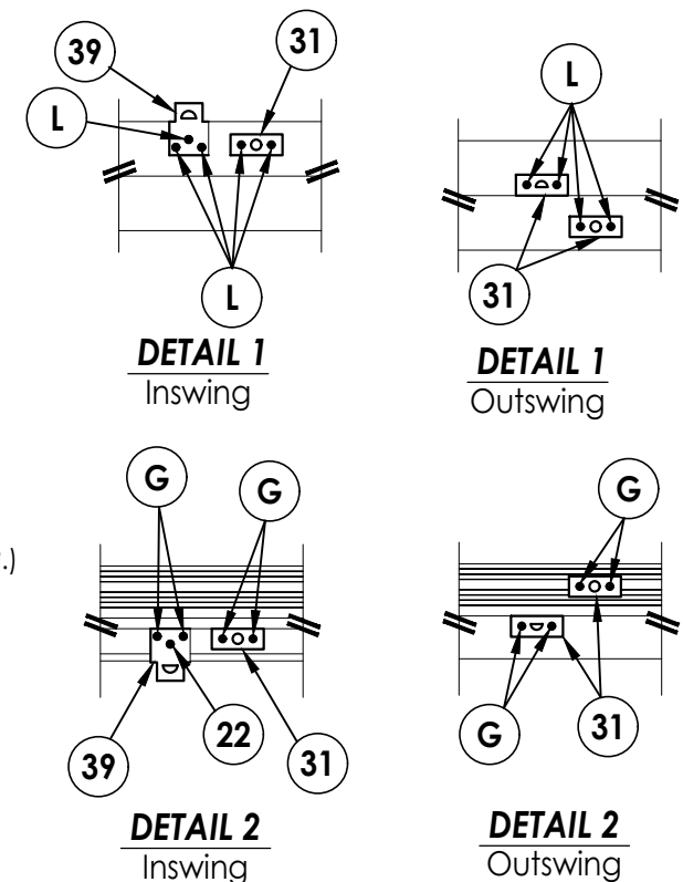
DOUBLE MULLION CLIP DETAIL
